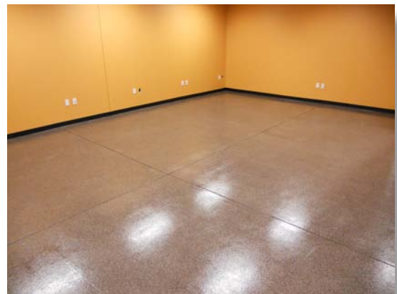
Two topcoats - 1/16" color chips
